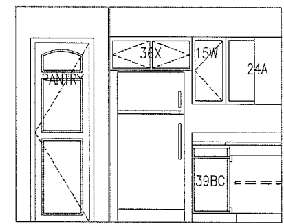
EAST ELEVATION
